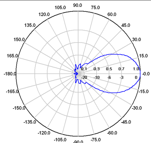
H-Ebene / H-Plane 3 GHz
