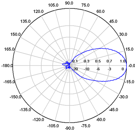
E-Ebene / E-Plane 2 GHz
