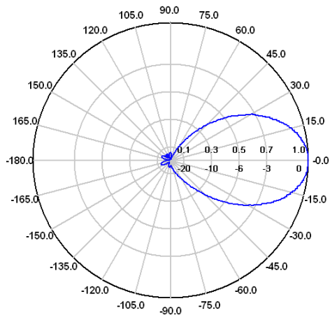
E-Ebene / E-Plane 1 GHz
