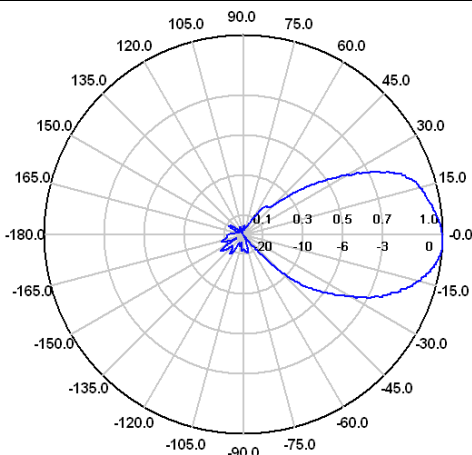
E-Ebene / E-Plane 3 GHz
